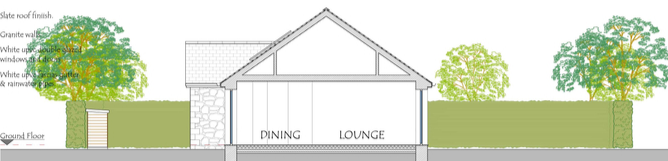
PROPOSED SOUTH ELEVATION/SECTION SCALE 1:100
