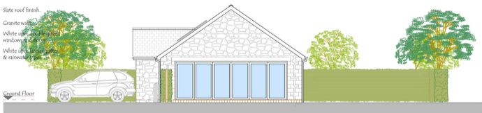
PROPOSED SOUTH ELEVATION SCALE 1:100
